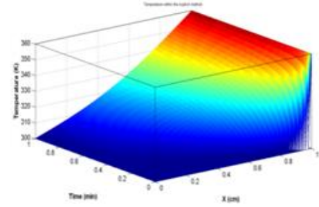
Fig.2.Scheme variation of the depth with temperature under duration time (2 minutes)
