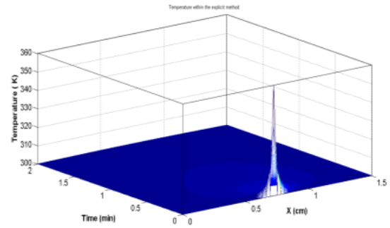
Fig.3.Color map for variation of the depth with temperature under duration time (1 minutes)
